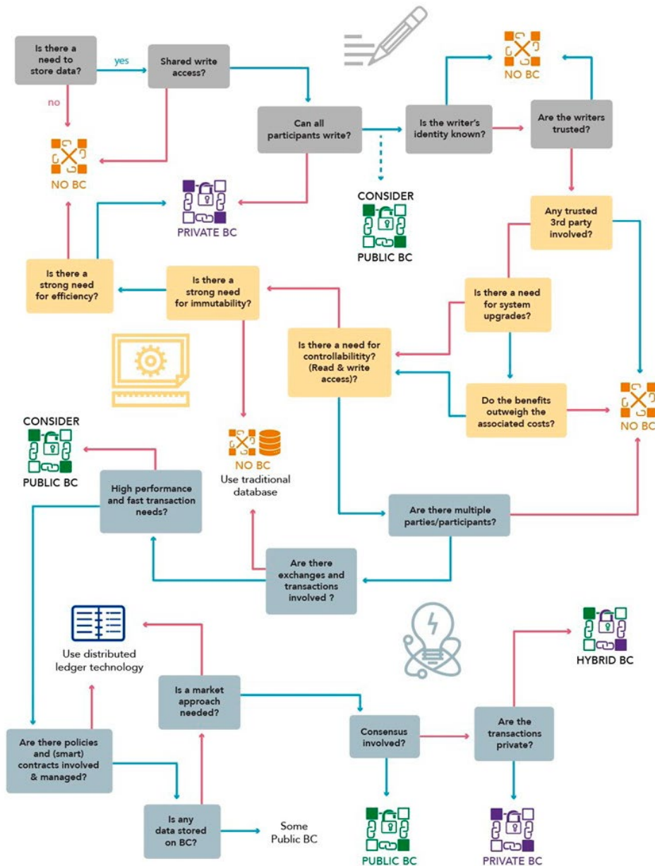
Fig. 2. Blockchain Roadmap. Source: Mylrea &amp; Gourisetti, 2018.
